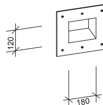
Perspective
