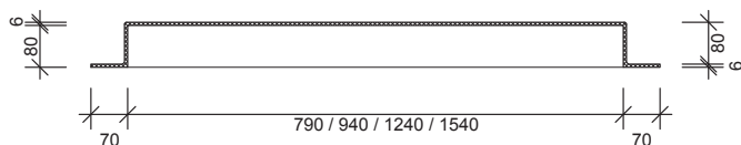
Section
