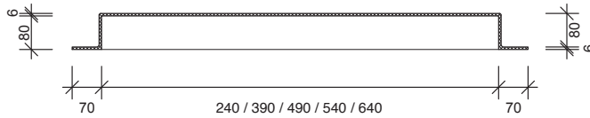
Section
