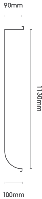
Side Elevation
