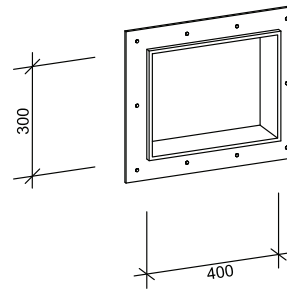
Perspective
